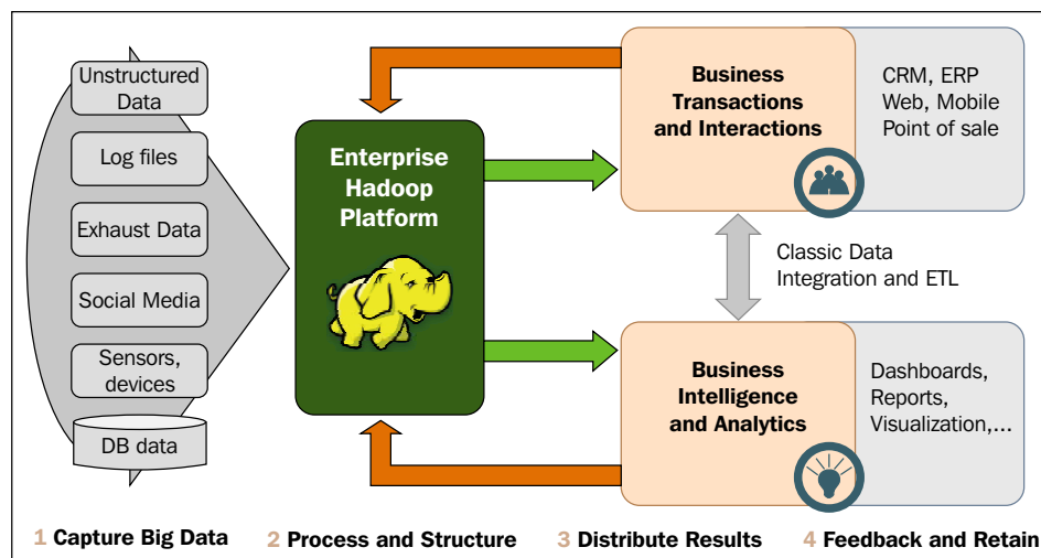
Hadoop basic data flow
